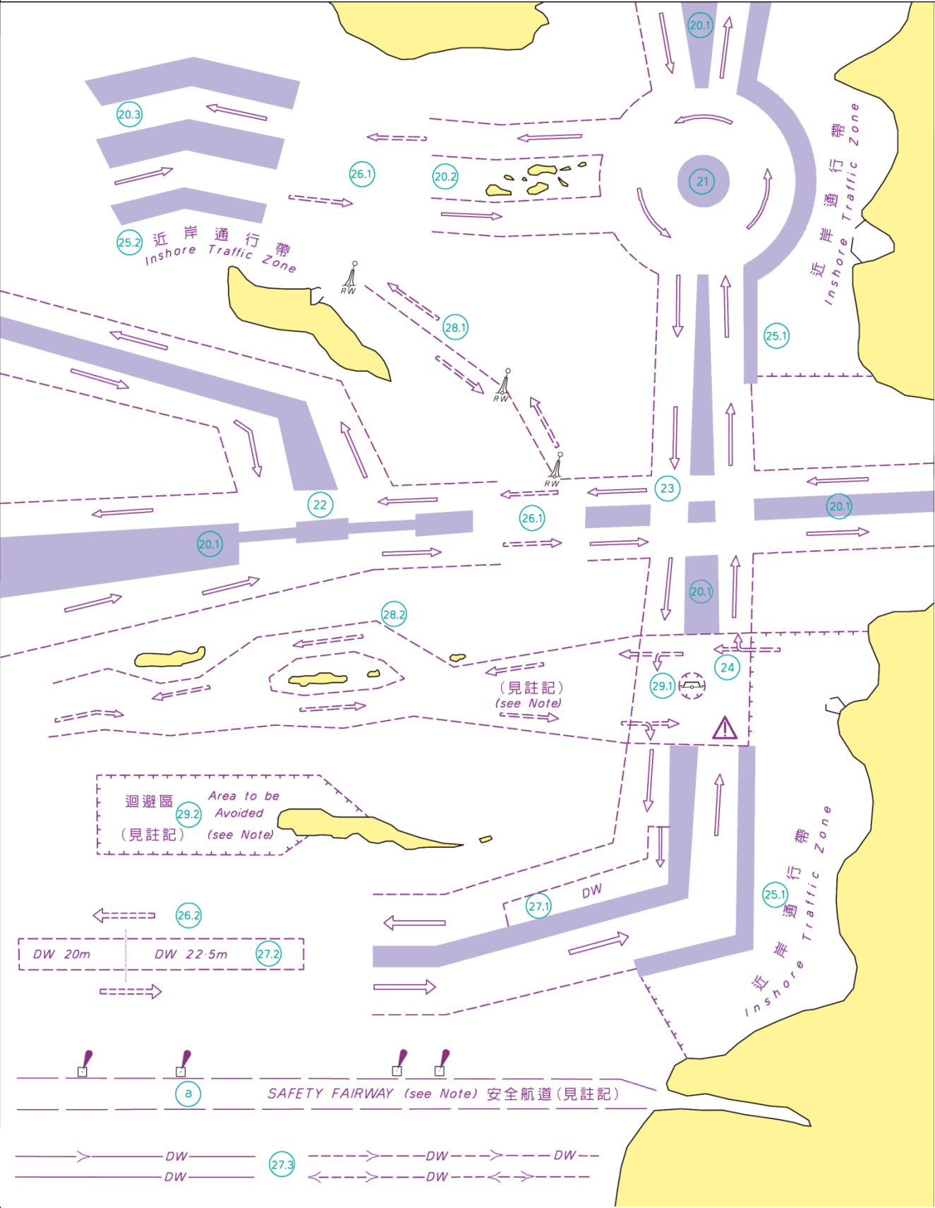
航道規劃示例 Examples of Routing Measures
